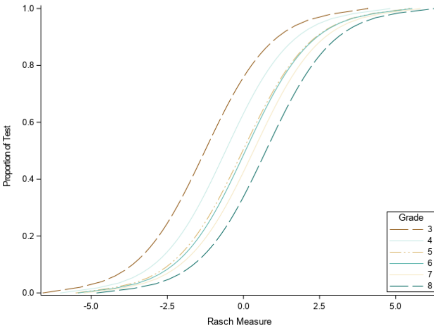
Figure 4.4. Test Characteristic Curve, Mathematics, Non-Accommodated Online Forms
