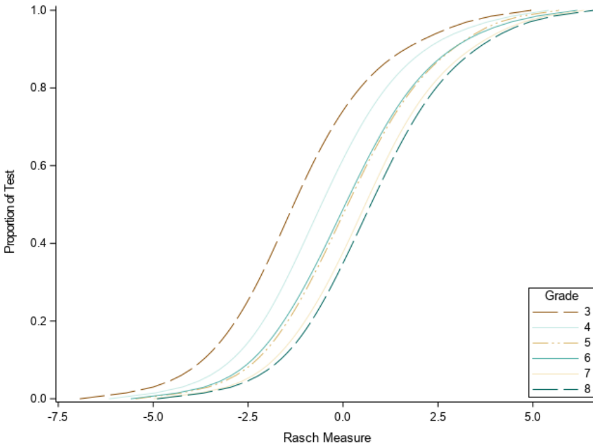
Figure 4.1. Test Characteristic Curve, ELA, Print and Accommodated Online Forms
