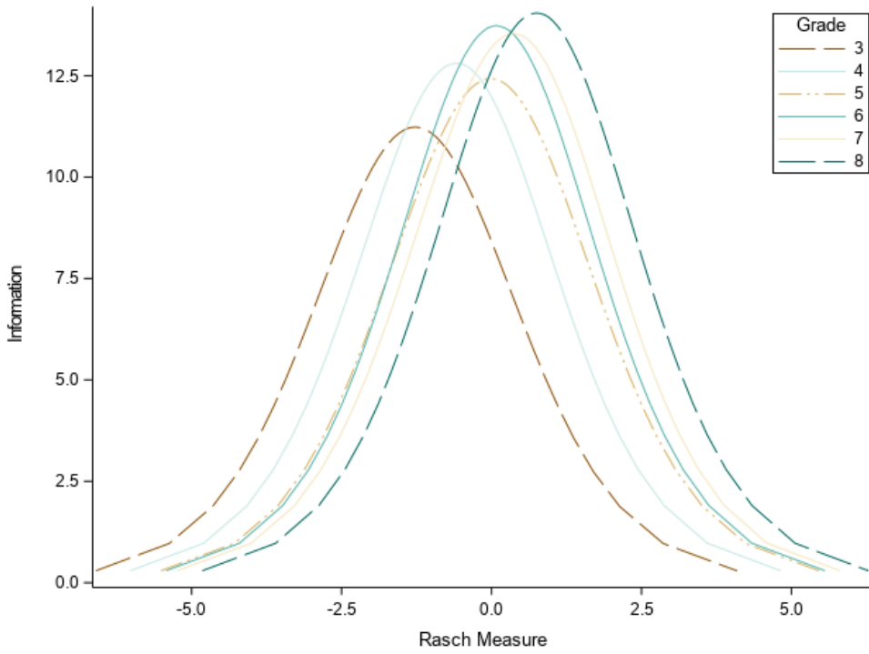
Figure 4.8. Test Information Functions, Mathematics, Non-Accommodated Online Forms
