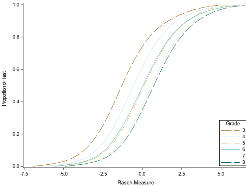
Figure 4.2. Test Characteristic Curve, ELA, Non-Accommodated Online Forms
