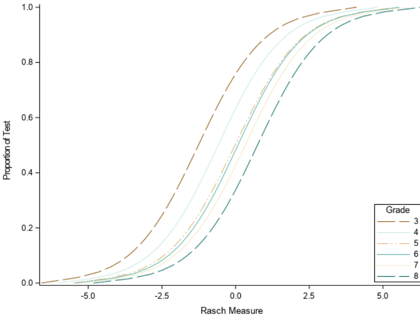
Figure 4.3. Test Characteristic Curve, Mathematics, Print and Accommodated Online Forms
