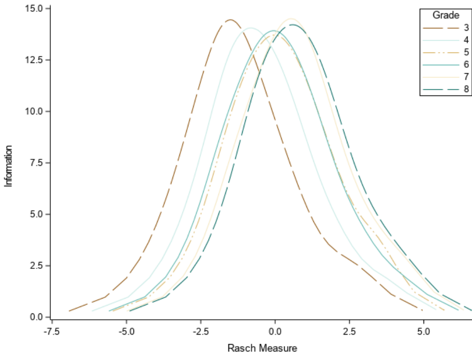
Figure 4.5. Test Information Functions, ELA, Print and Accommodated Online Forms
