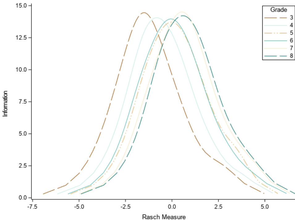
Figure 4.6. Test Information Functions, ELA, Non-Accommodated Online Forms
